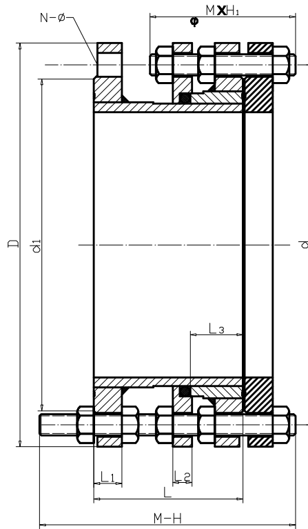
Dimensions(mm)
